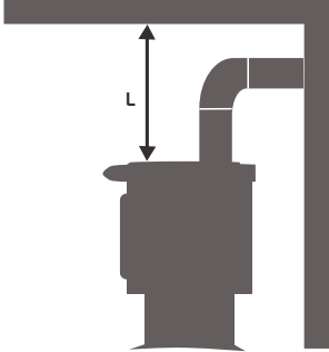
STOVE TO CEILING INSTALLATION
