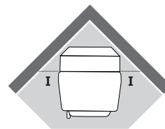
CLEARANCES* (CORNER INSTALLATION)
